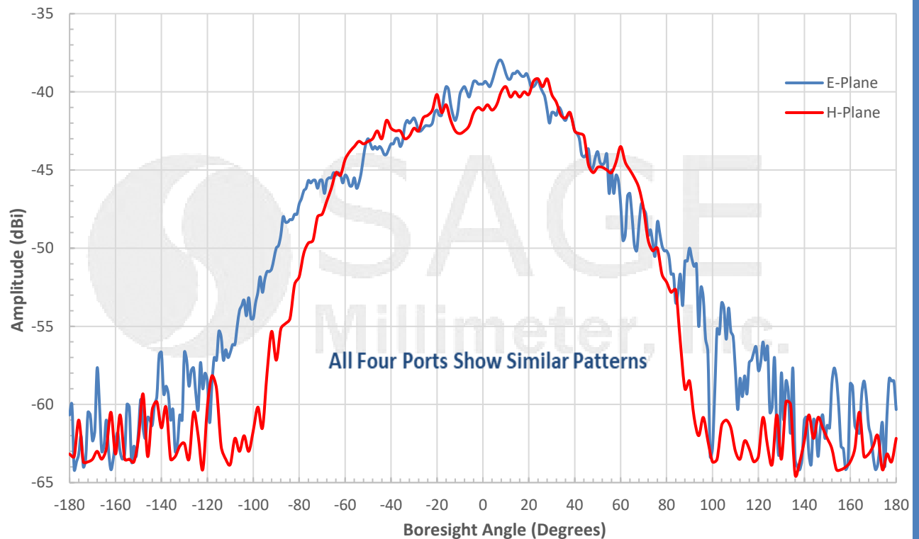
Measured Individual Patch Pattern @ 66.96 GHz
