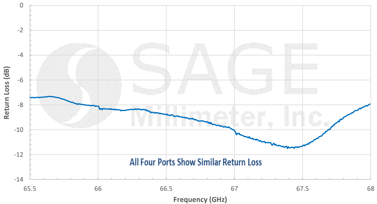
Measured Individual Patch Return Loss vs. Frequency
