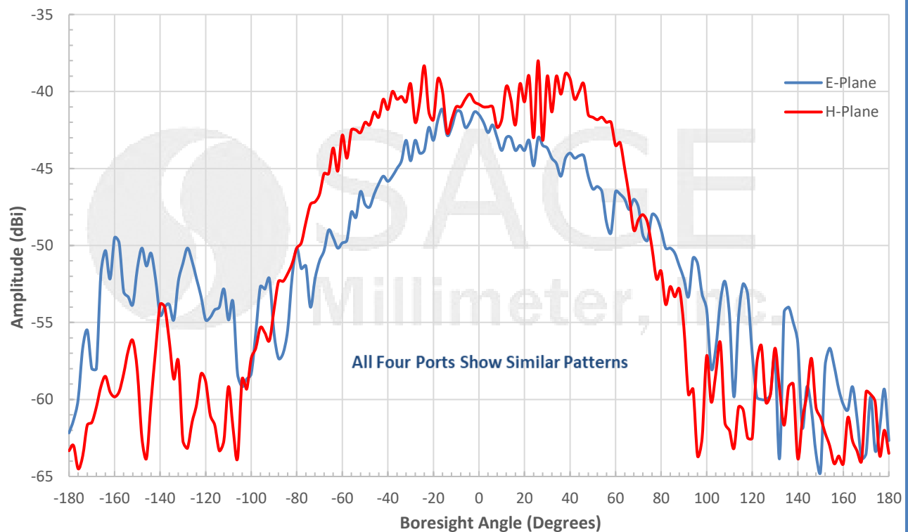
Measured Individual Patch Pattern @ 64.8 GHz
