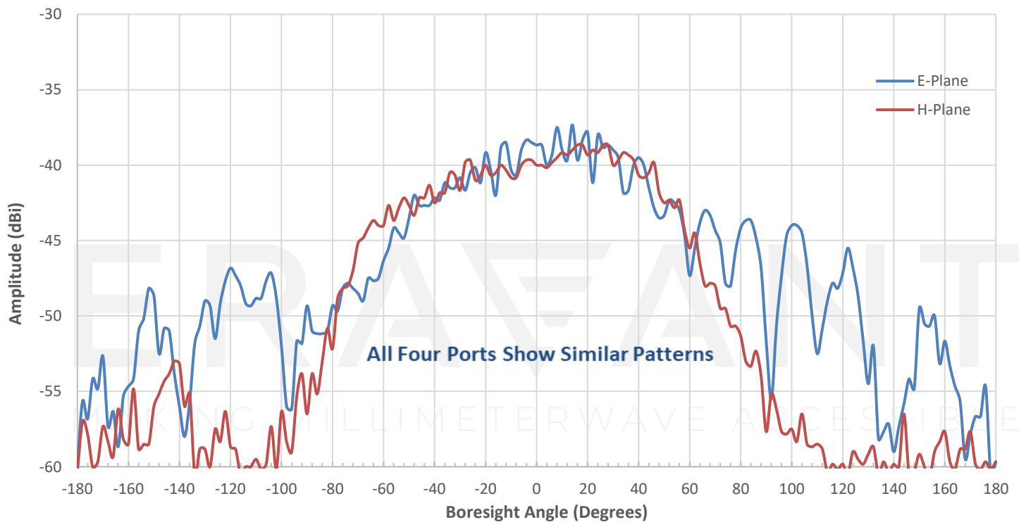
Measured Individual Patch Pattern @ 62.64 GHz
