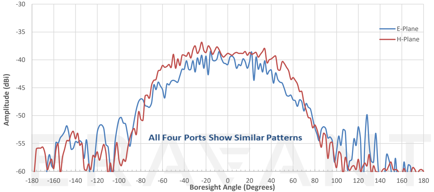
Measured Individual Patch Pattern @ 62.64 GHz
