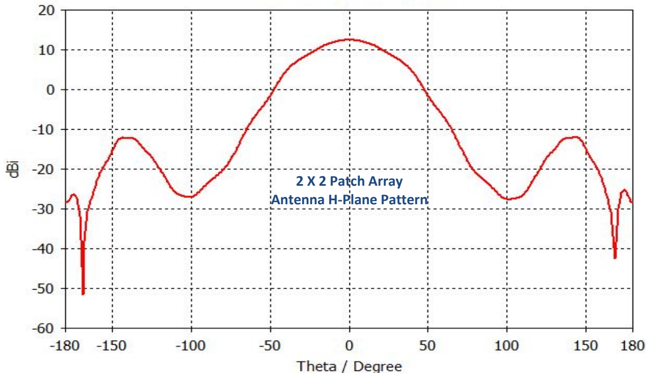
Farfield Directivity Abs (Phi=0)
