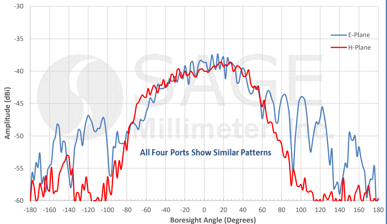
Measured Individual Patch Pattern @ 62.64 GHz
