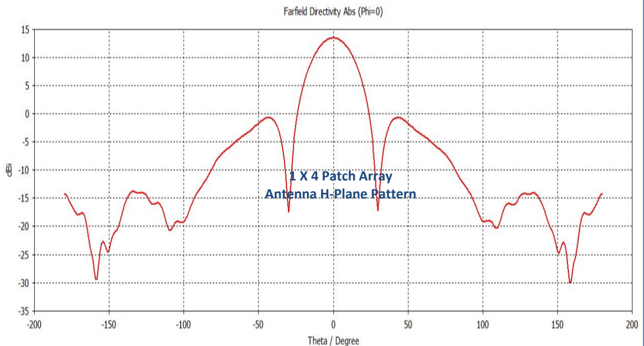
In-Phase Fed Simulated H-Plane Patch Array Antenna Pattern @ 63 GHz
