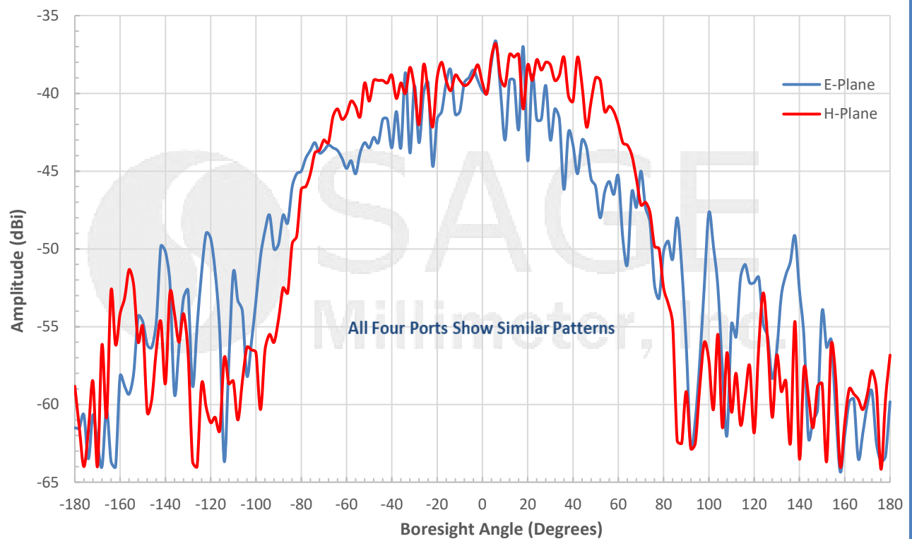
Measured Individual Patch Pattern @ 62.64 GHz
