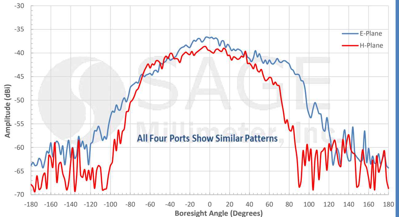
Measured Individual Patch Pattern @ 62.64 GHz
