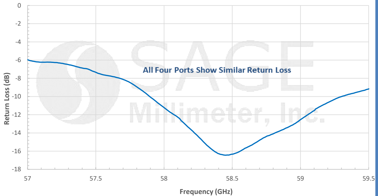
Measured Individual Patch Return Loss vs. Frequency
