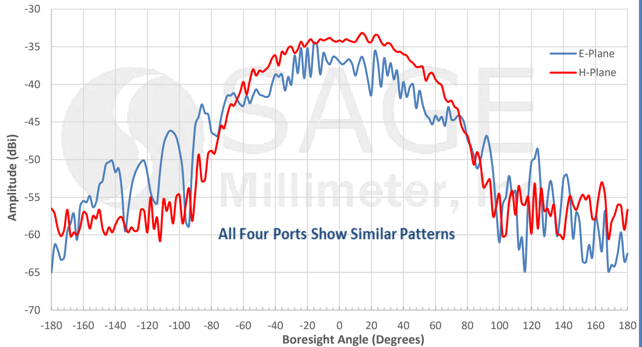
Measured Individual Patch Pattern @ 58.32 GHz
