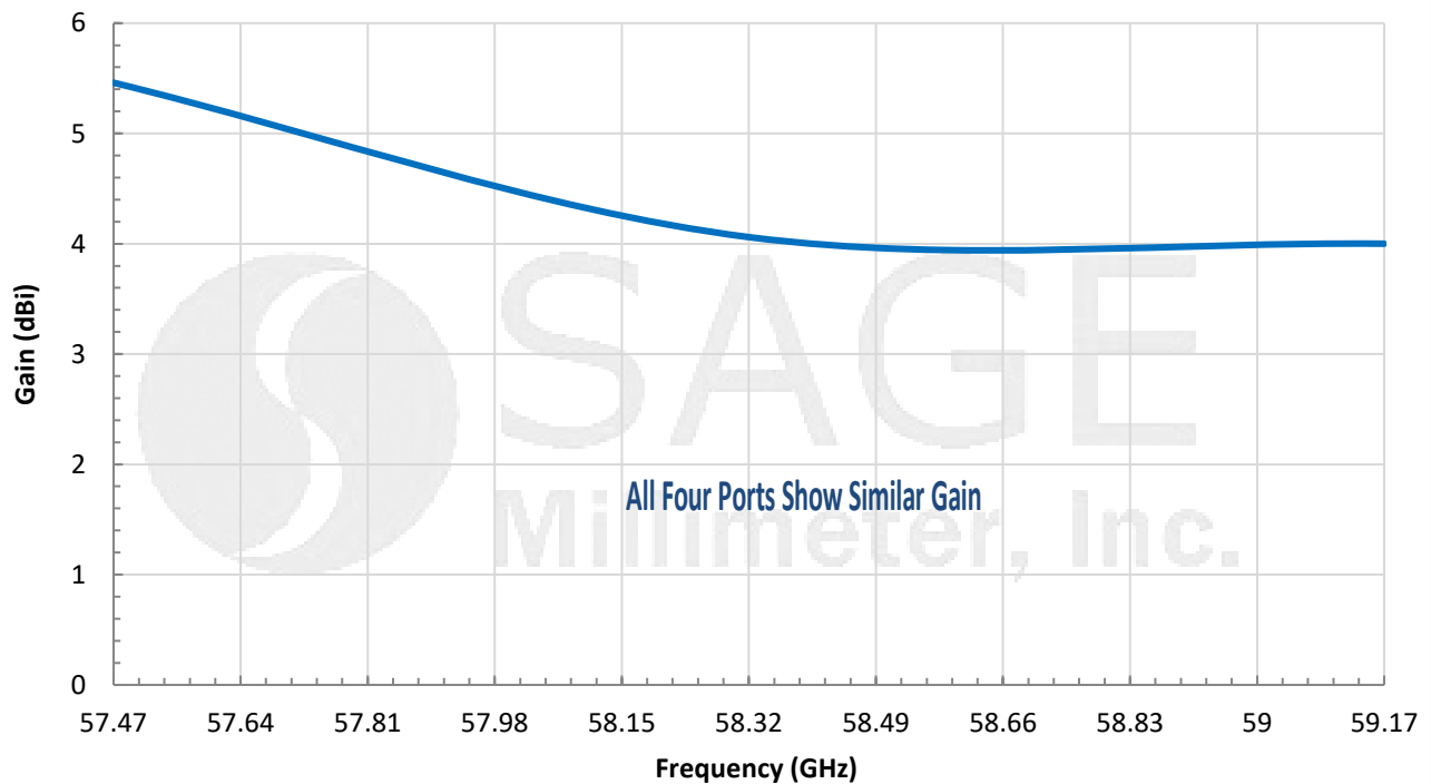
Measured Individual Patch Gain vs. Frequency
