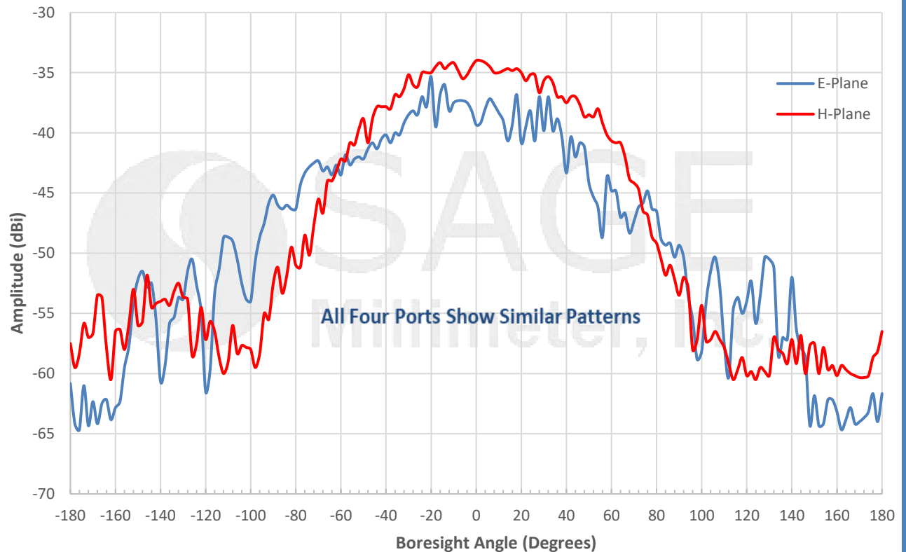
Measured Individual Patch Pattern @ 58.32 GHz
