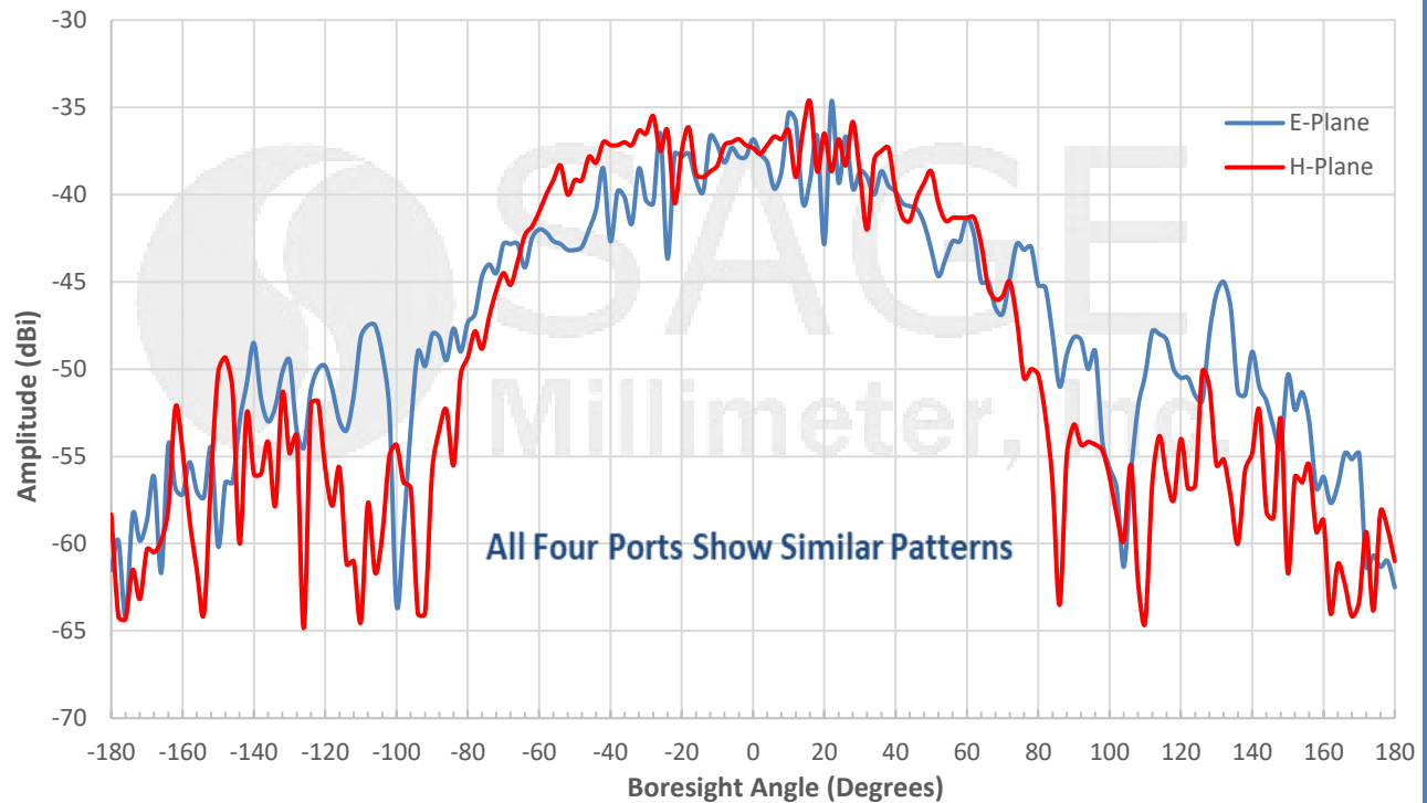
Measured Individual Patch Pattern @ 58.32 GHz
