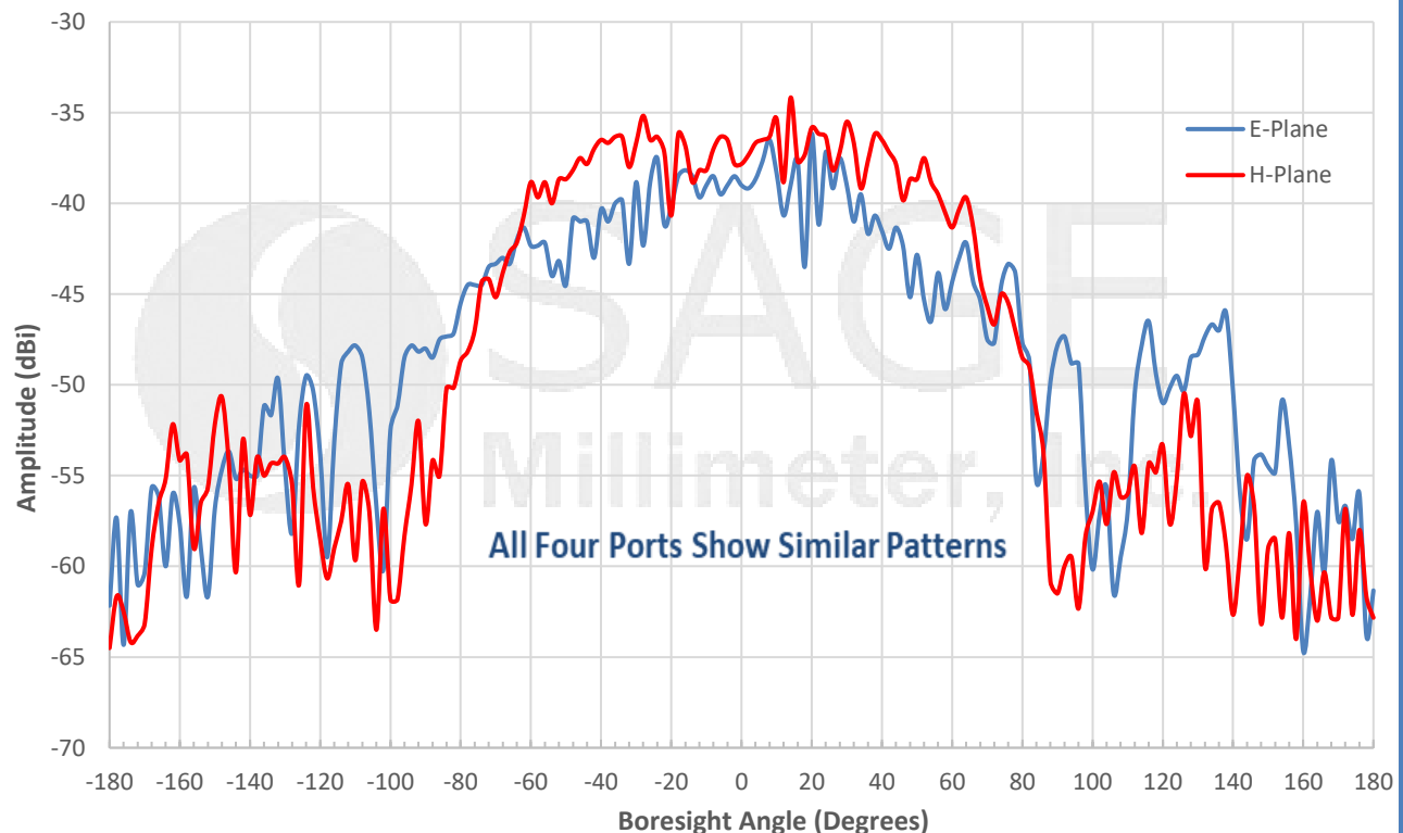
Measured Individual Patch Pattern @ 58.32 GHz
