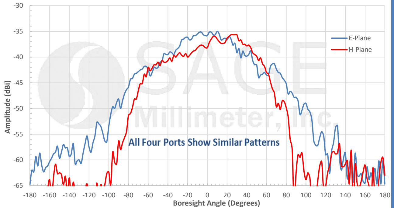
Measured Port 1 E-Plane Antenna Pattern @ 58.32 GHz
