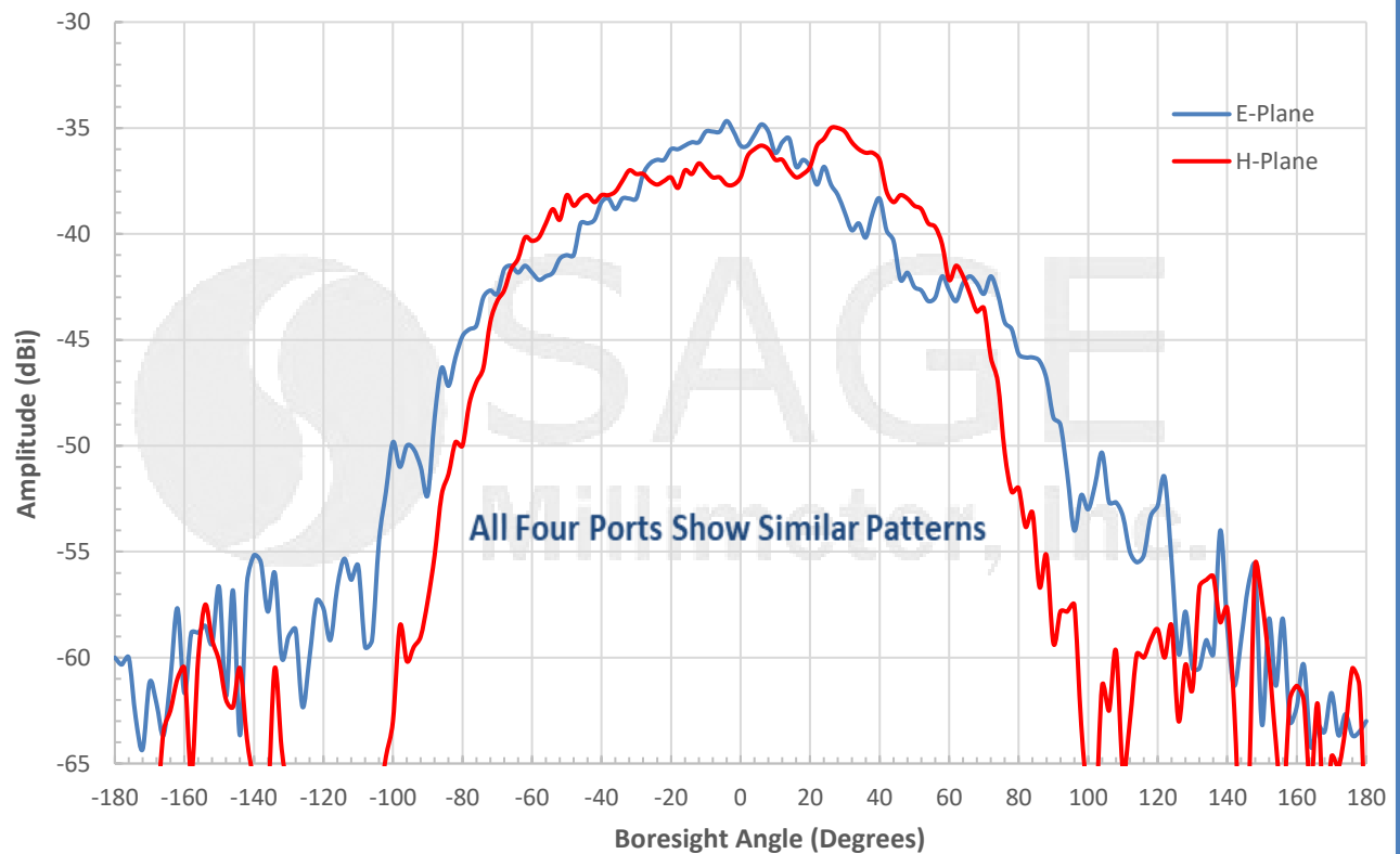
Measured Port 1 E-Plane Antenna Pattern @ 58.32 GHz
