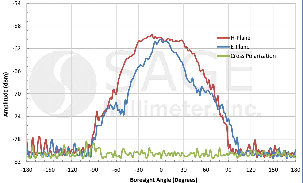
Measured Antenna Patterns for Port 2 & 3 @ 39 GHz
