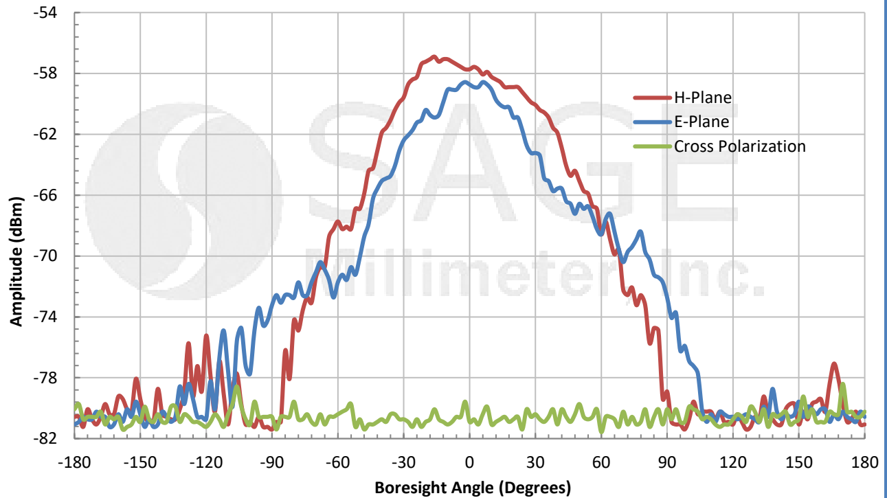
Measured Antenna Patterns for Port 2 & 3 @ 39 GHz
