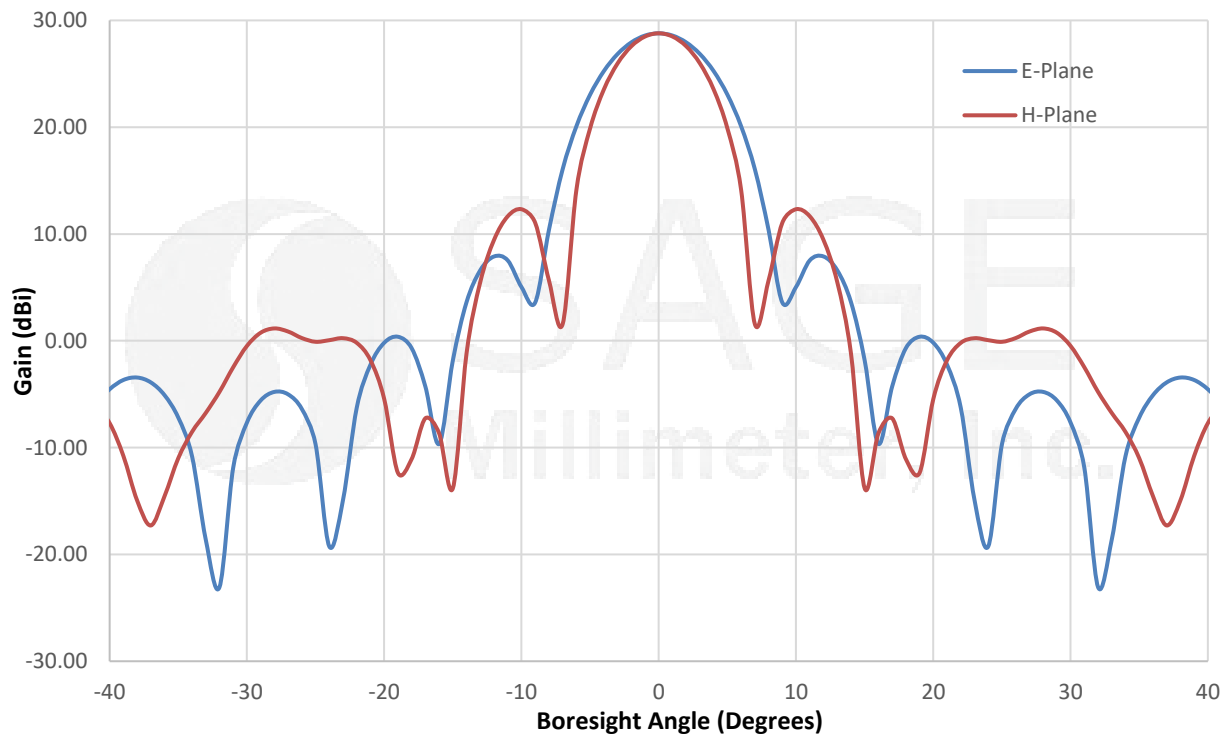
Simulated Antenna Pattern @ 75 GHz
