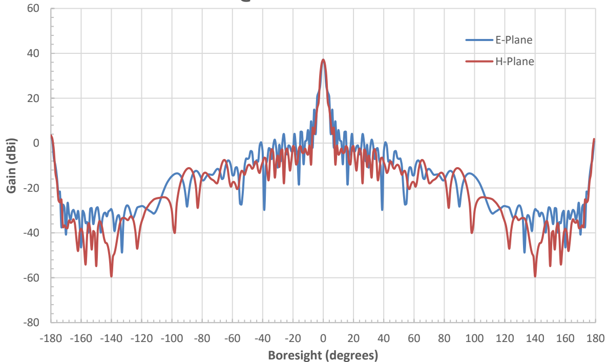
Simulated Antenna Patterns @ 78.5 GHz
