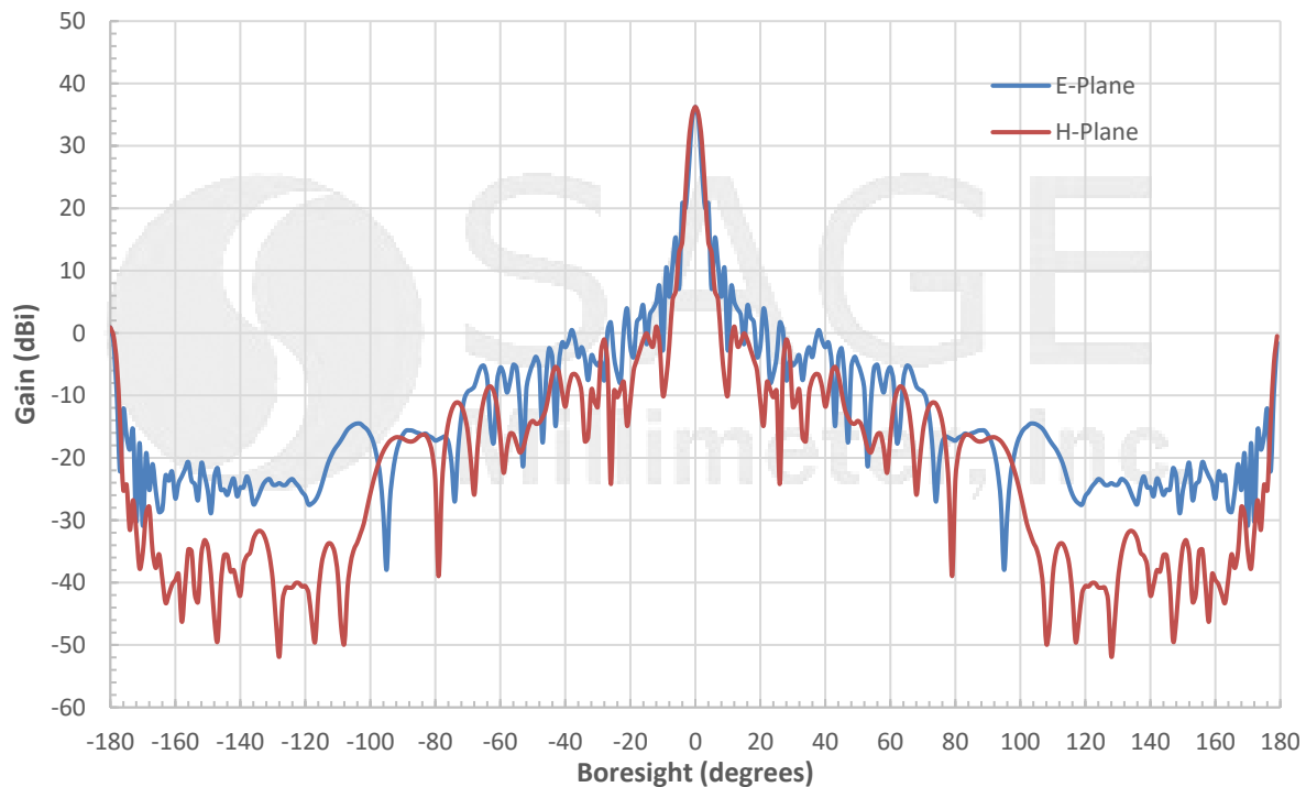
Simulated Antenna Patterns @ 71 GHz
