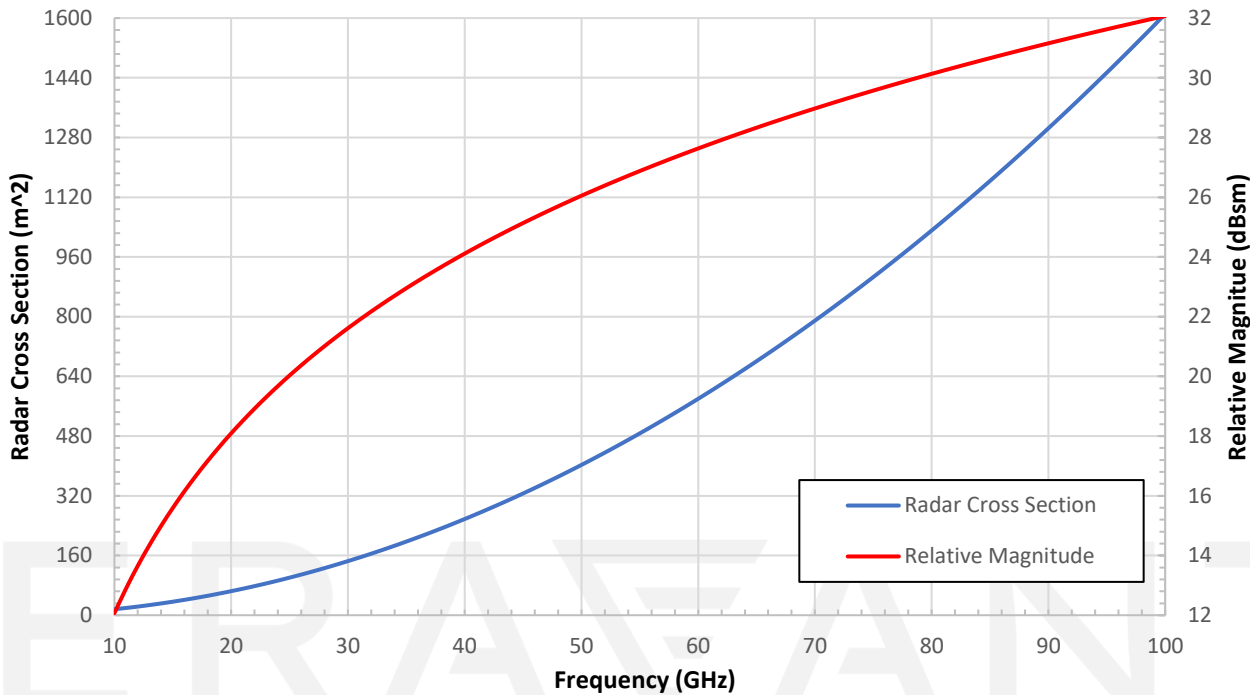
Calculated Radar Cross Section and Relative Magnitude
