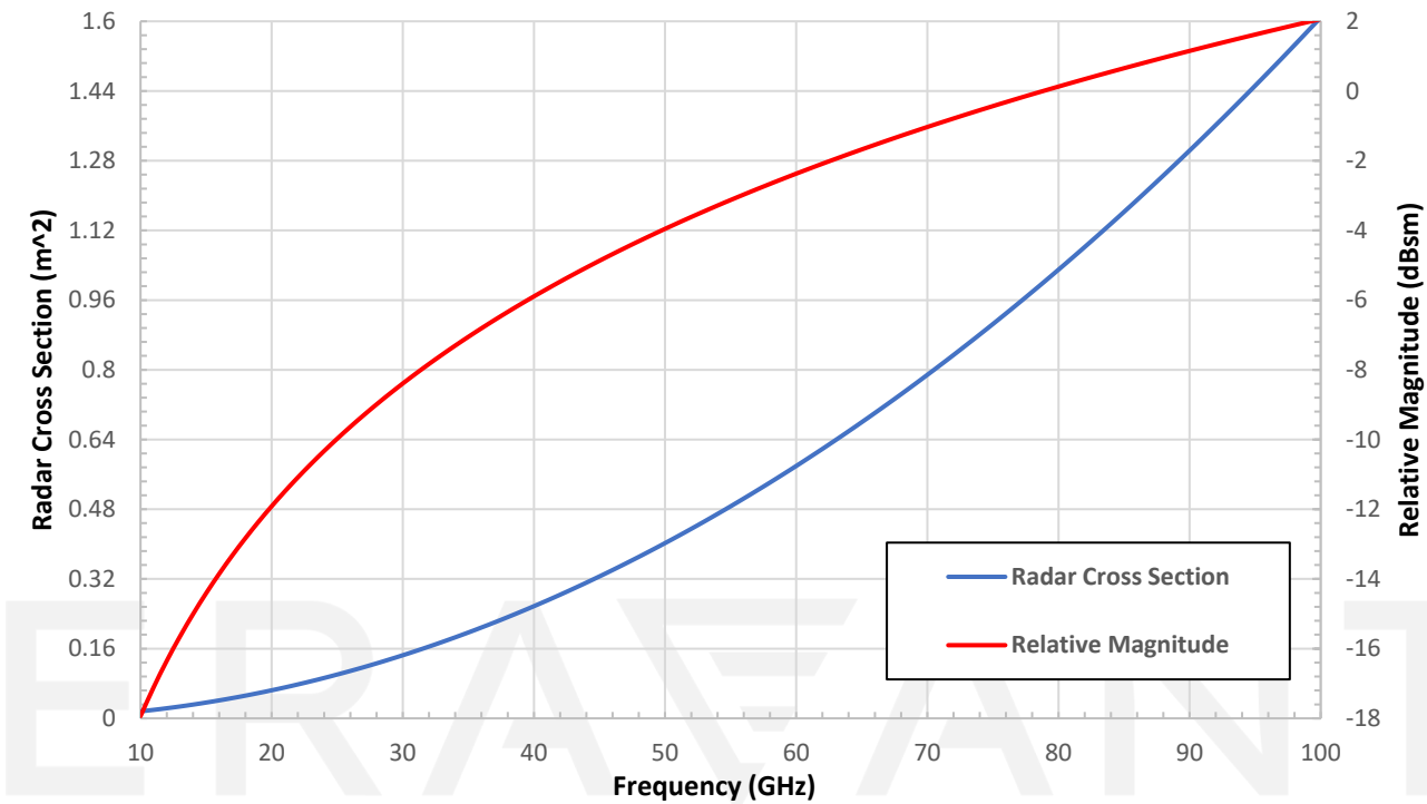
Calculated Radar Cross Section and Relative Magnitude
