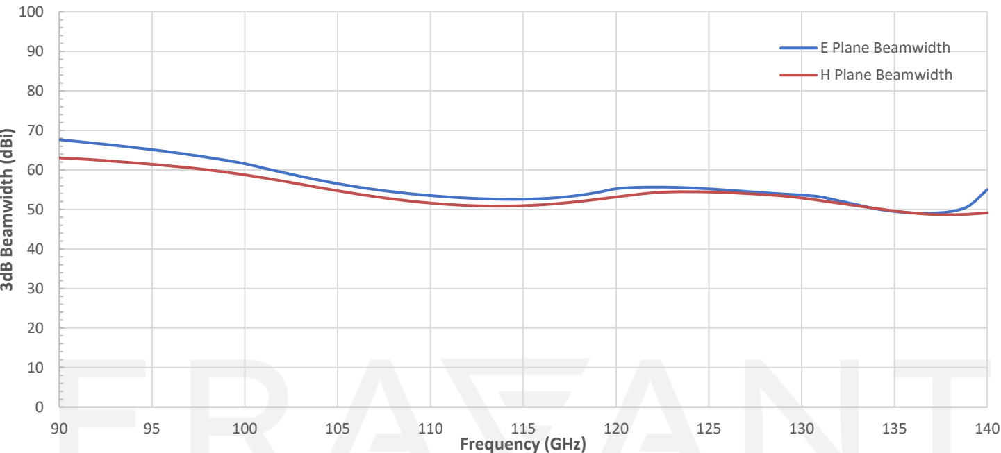
Simulated 3dB Beamwidth vs Frequency
