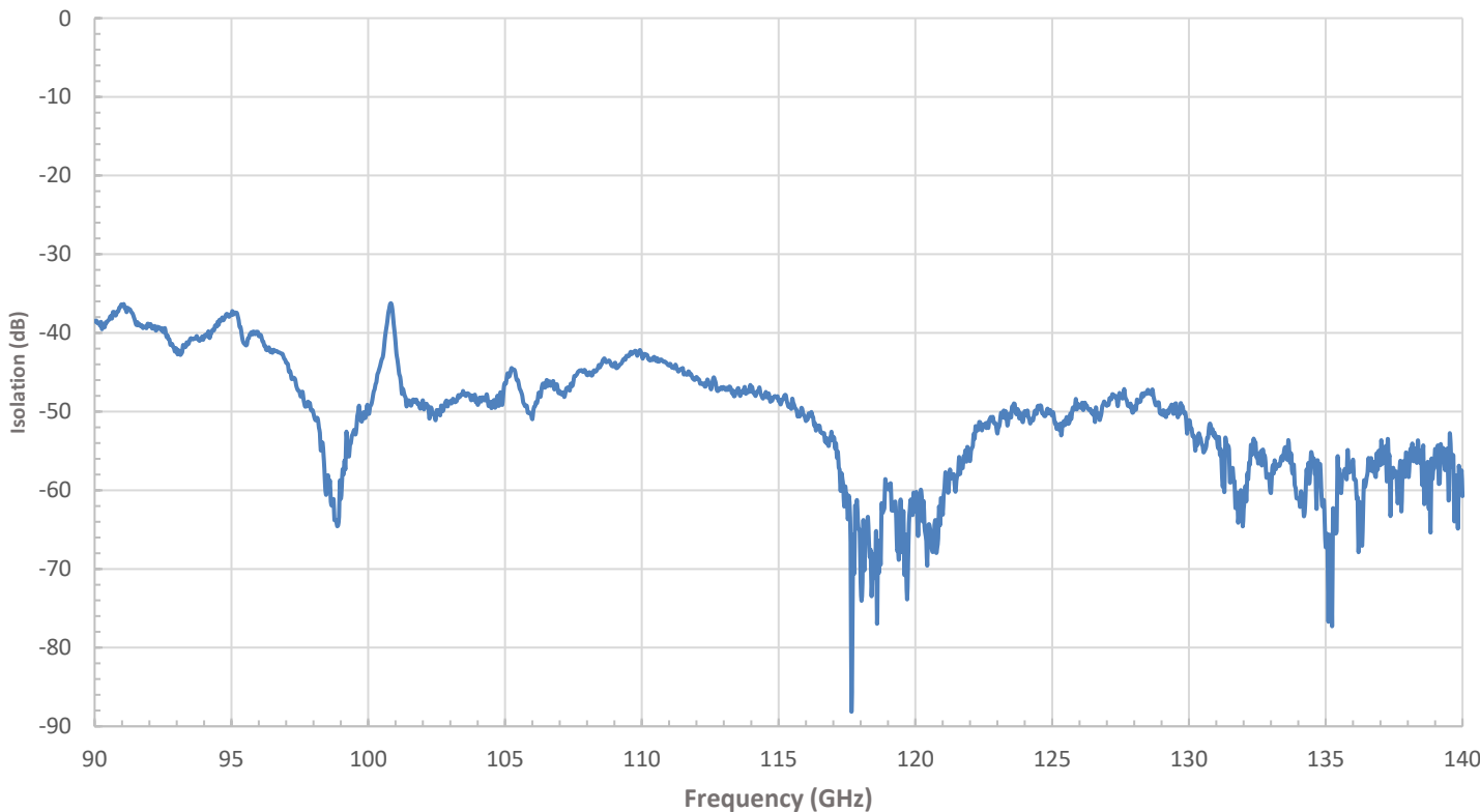
Typical Isolation Vs Frequency
