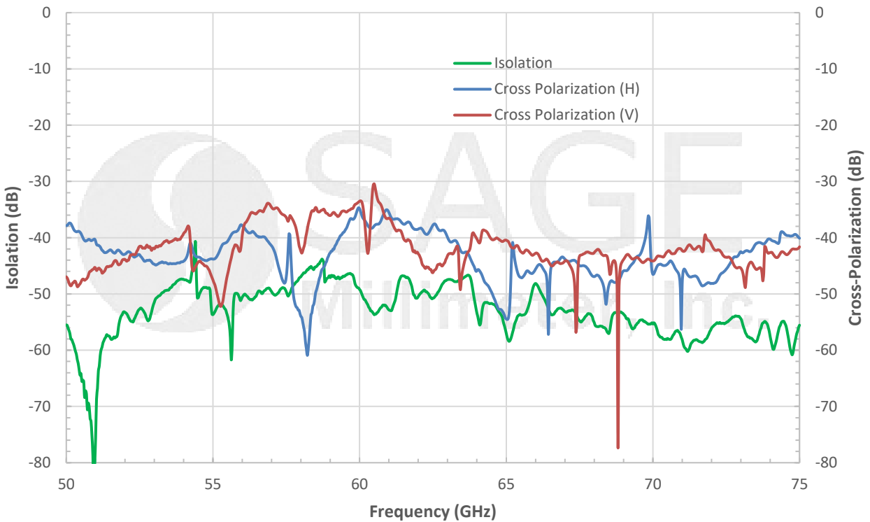
Typical Isolation and Cross Polarization vs Frequency
