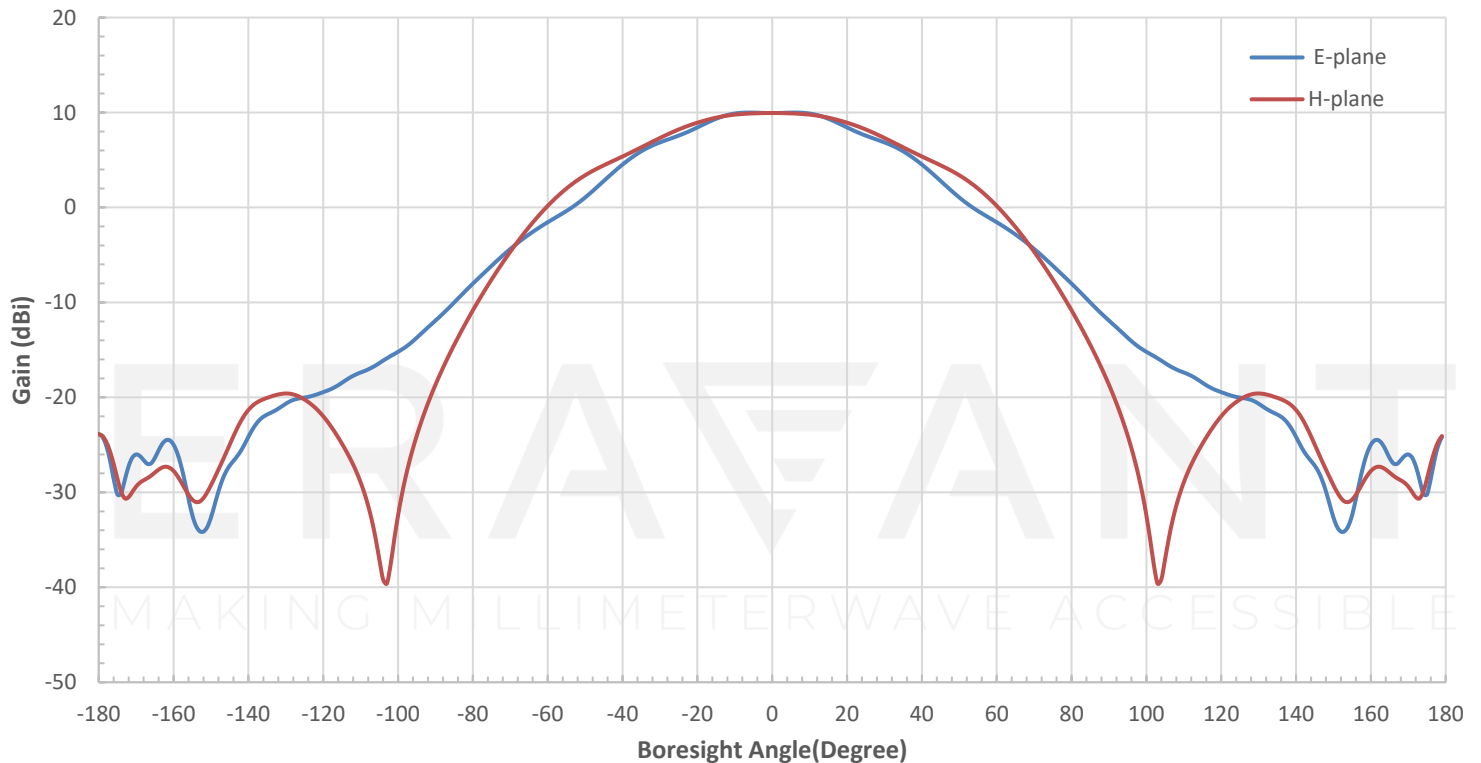
Simulated Pattern @ 41.5 GHz
