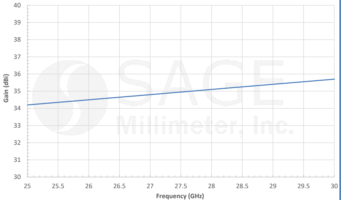
Simulated Gain vs. Frequency
