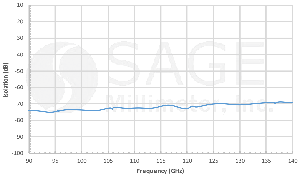
Simulated Isolation vs. Frequency
