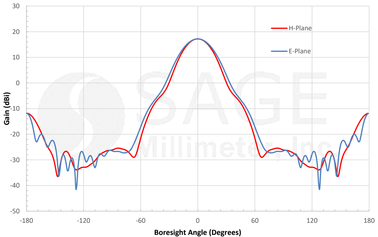
Simulated Antenna Patterns @ 140 GHz
