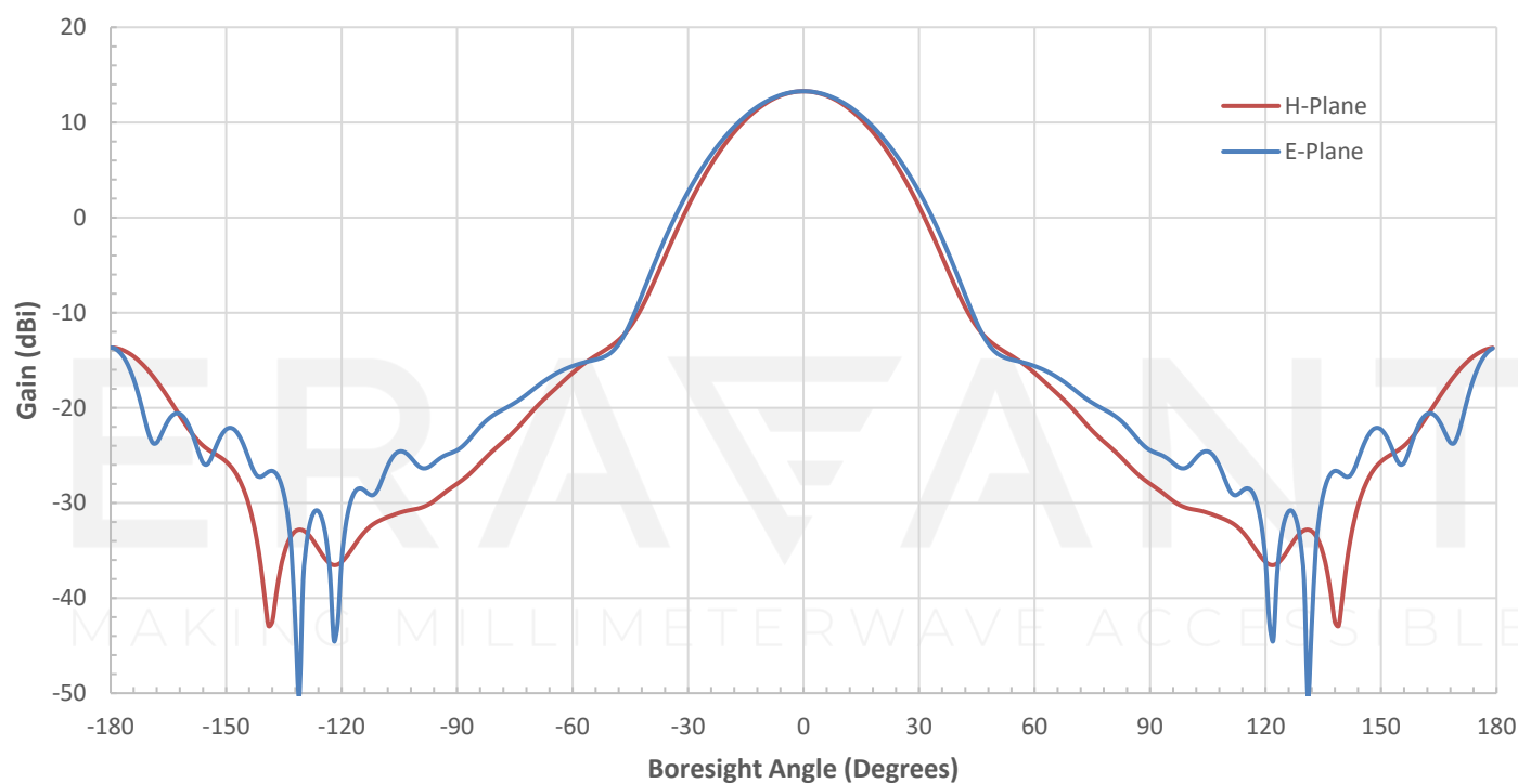
Simulated Antenna Patterns @ 140 GHz
