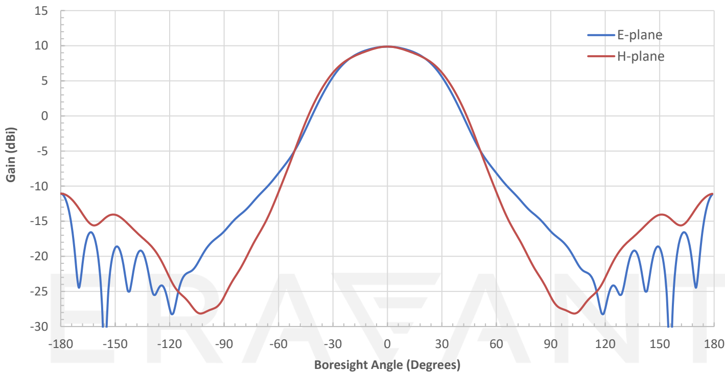
Simulated Antenna Patterns @ 170 GHz
