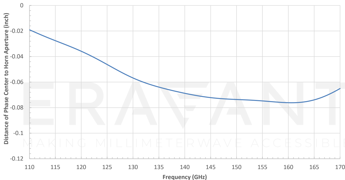
Simulated Phase Center vs. Frequency
