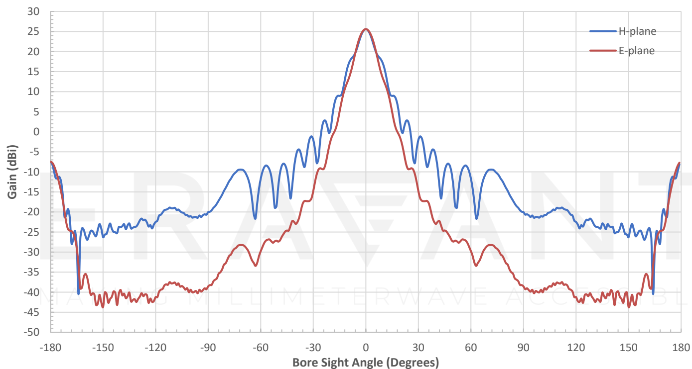
Simulated Antenna Pattern at 180 GHz
