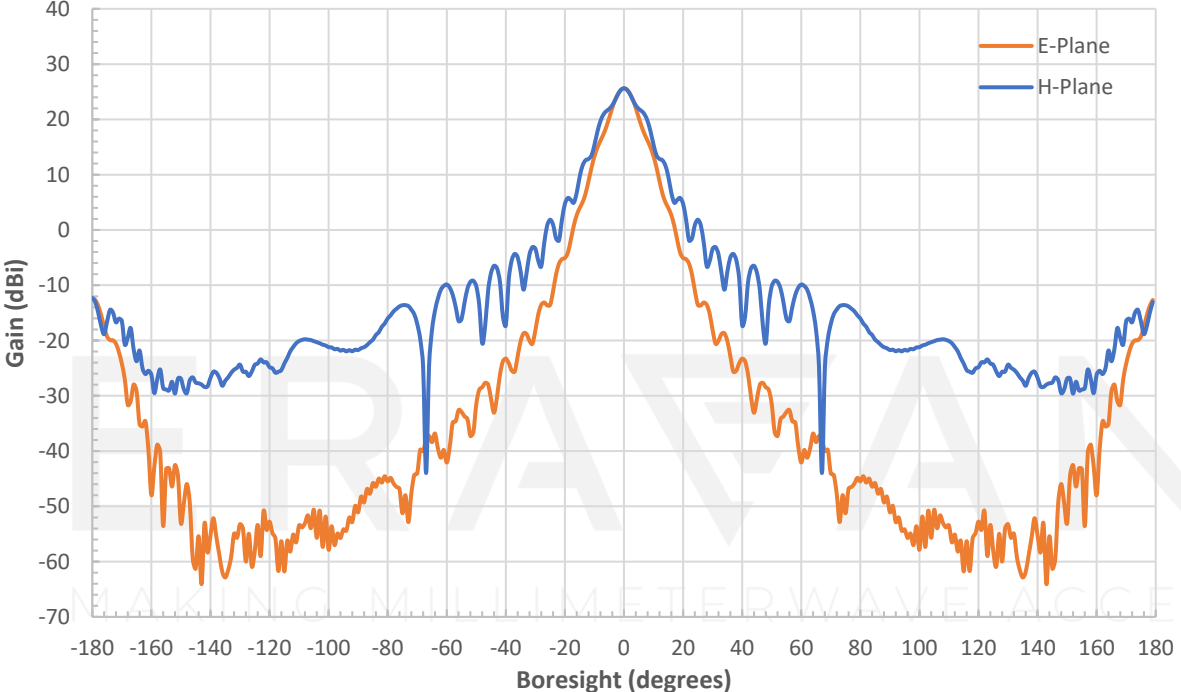
Simulated Antenna Patterns @ 272.5 GHz
