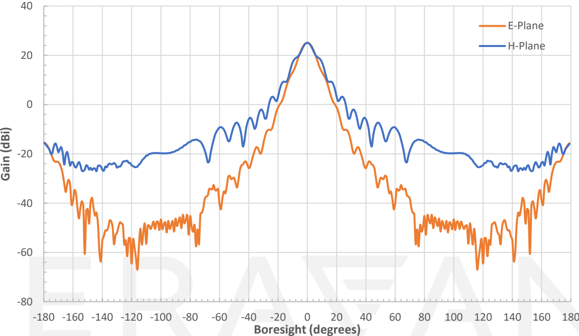
Simulated Antenna Patterns @ 220 GHz
