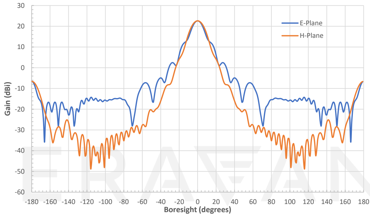
Simulated Antenna Patterns @ 33 GHz
