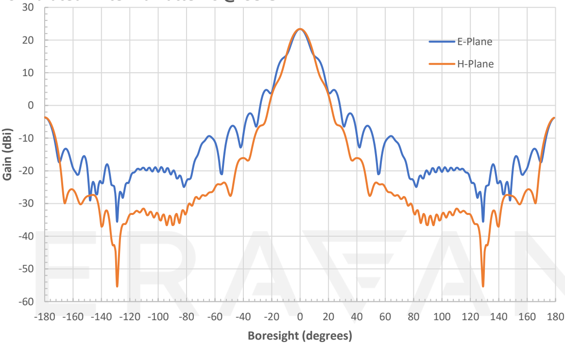
Simulated Antenna Patterns @ 38 GHz
