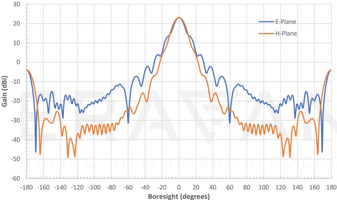
Simulated Antenna Patterns @ 35.5 GHz
