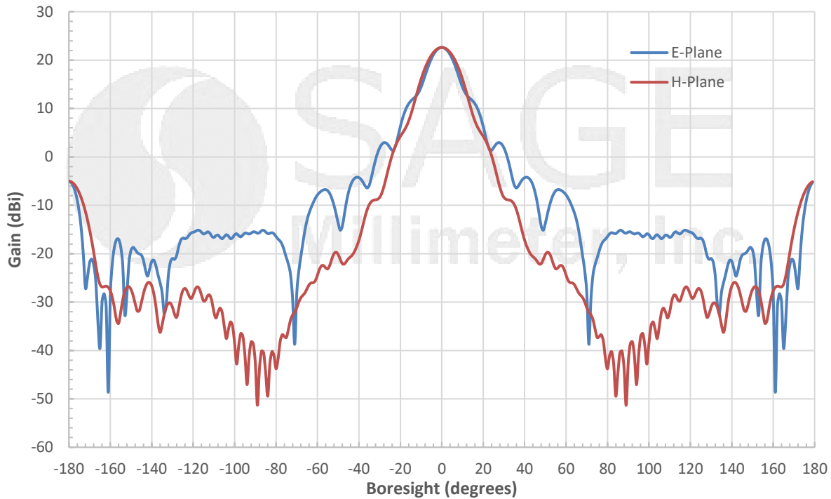
Simulated Antenna Patterns @ 58 GHz
