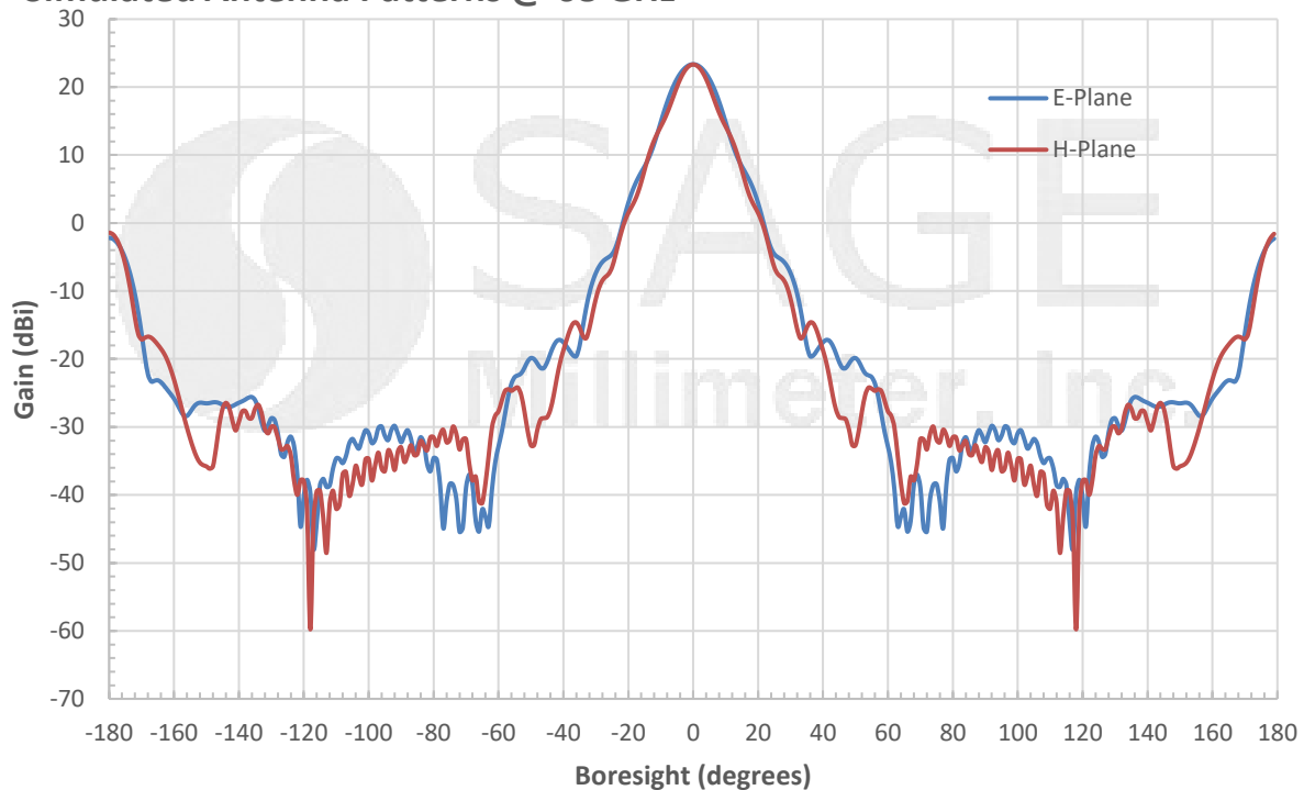
Simulated Antenna Patterns @ 68 GHz
