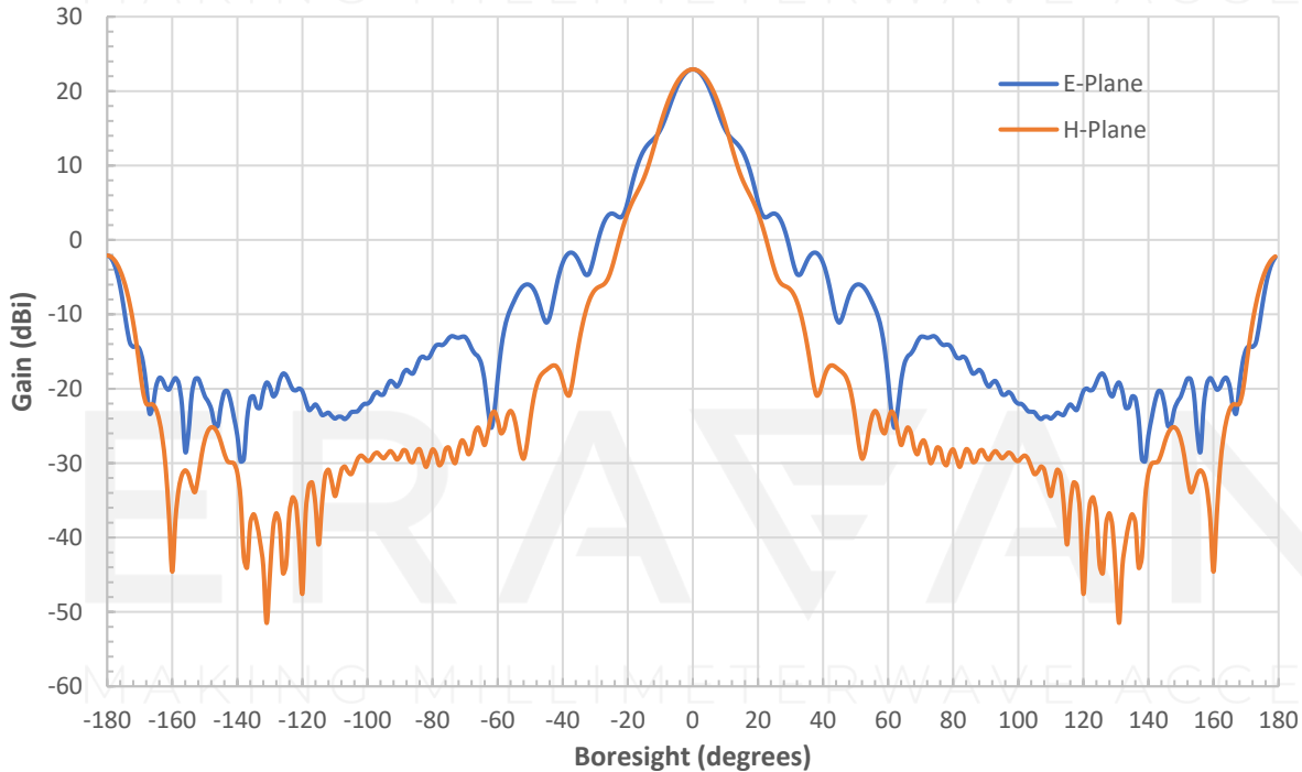
Simulated Antenna Patterns @ 82 GHz
