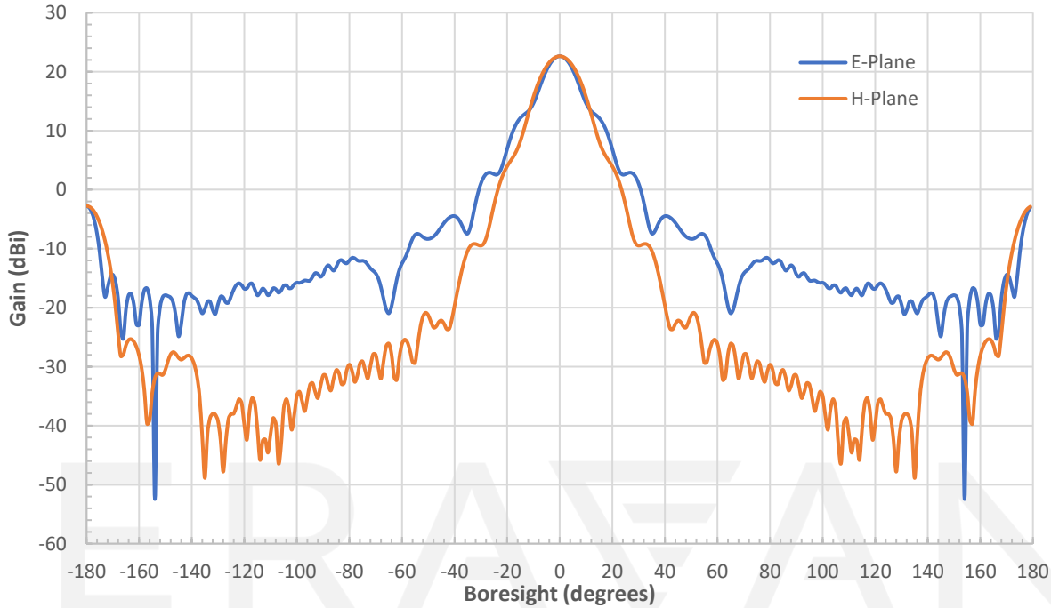
Simulated Antenna Patterns @ 77 GHz
