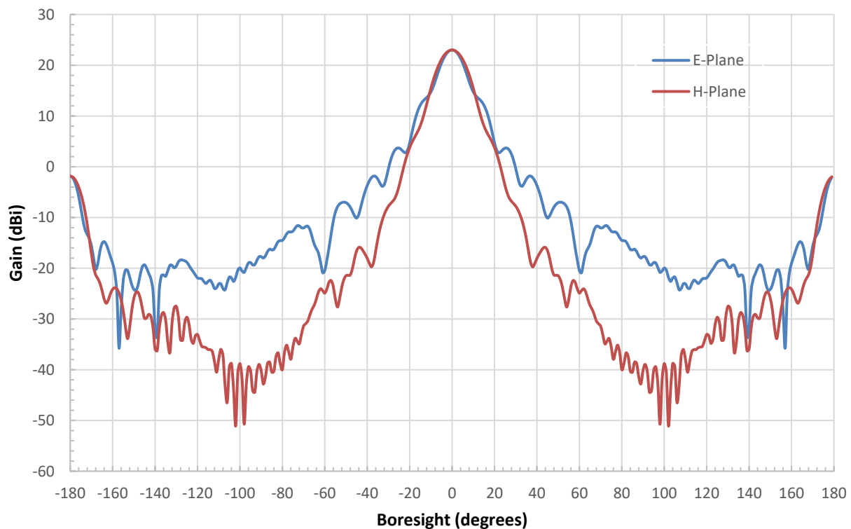
Simulated Antenna Patterns @ 93.5 GHz
