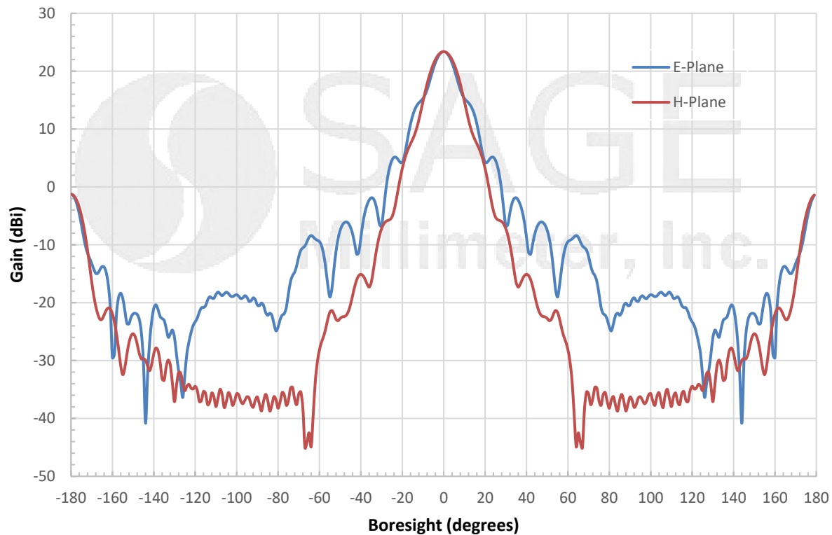
Simulated Antenna Patterns @ 100 GHz
