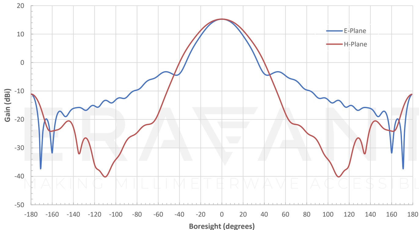
Simulated Antenna Patterns @ 46.5 GHz
