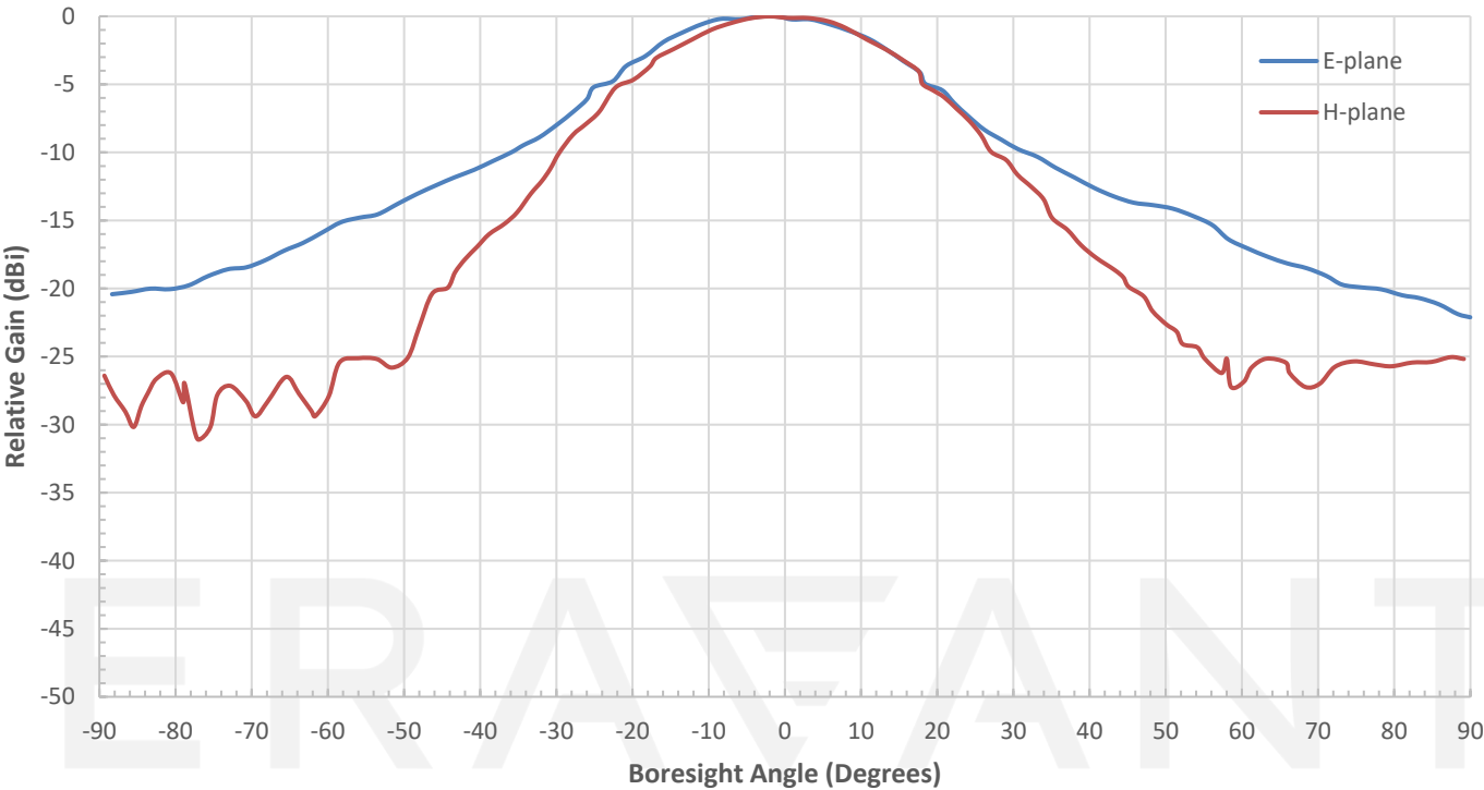
Typical Antenna Pattern @ 6 GHz
