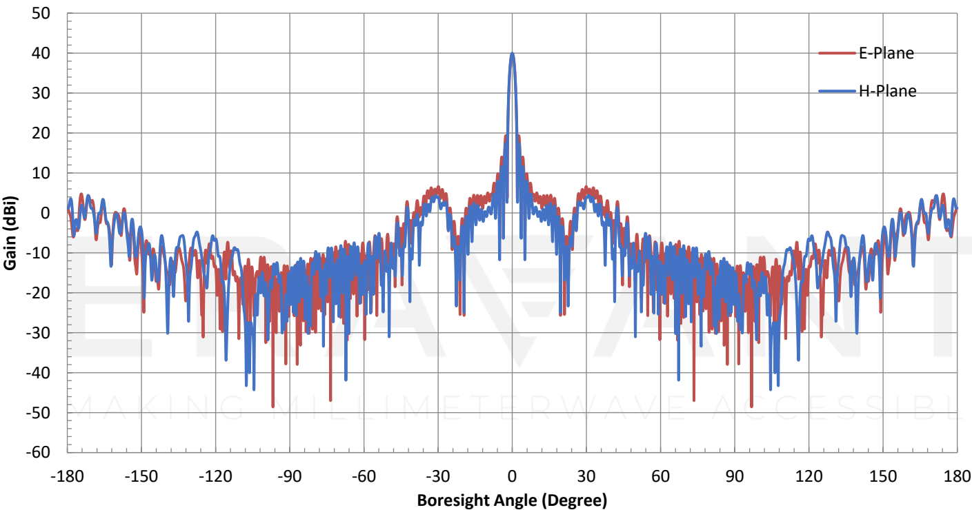
Simulated Antenna Pattern @ 145 GHz
